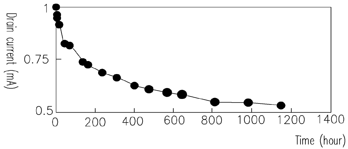
FIG. 4 (PRIOR ART)
